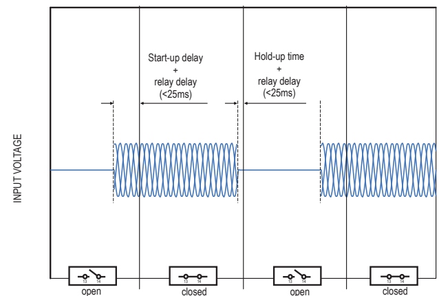
Fig. 22: DC-OK relay status in dependence of AC mains connection
