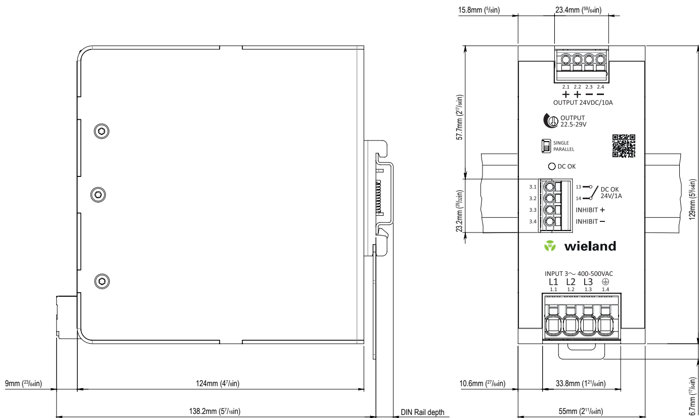
Fig. 18: Dimension drawing of DRB240-24-3-A1
