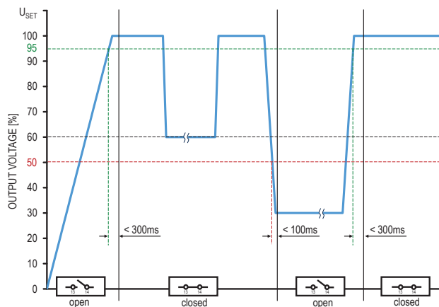
Fig. 21: DC-OK relay status in dependence of output voltage changes
