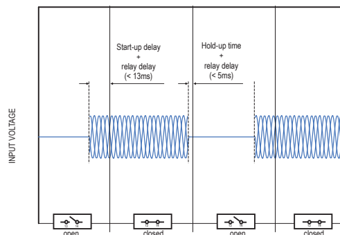
Fig. 22: DC-OK relay status in dependence of input voltage
