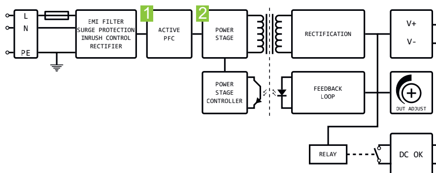
Fig. 25: Block diagram of P/C models
