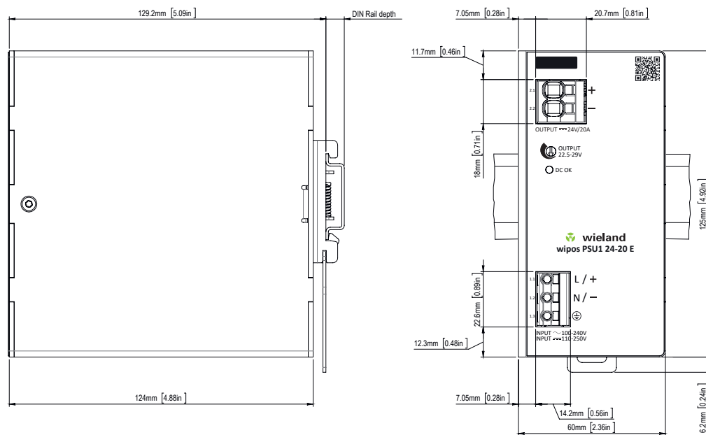
Fig. 17: Dimension drawing of wipos PSU1 24-20 E
