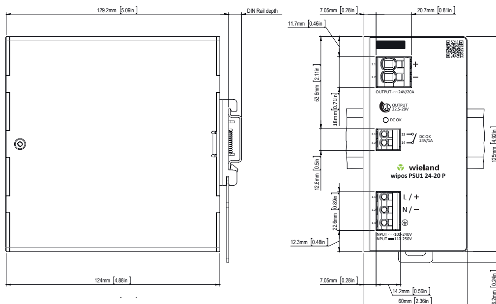
Fig. 18: Dimension drawing of wipos PSU1 24-20 P/C
