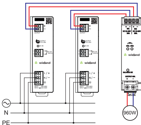
Fig. 27: Connection scheme of power supplies in parallel for the purpose of output power increase
