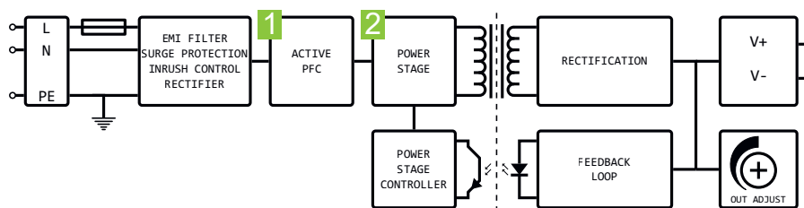
Fig. 24: Block diagram of E models
