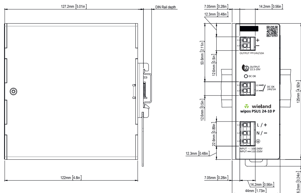
Fig. 17: Dimension drawing of wipos PSU1 24-10 P/C
