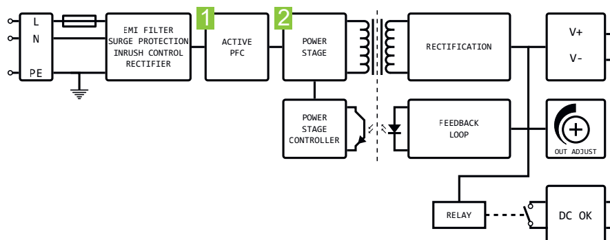
Fig. 24: Block diagram of P/C models
