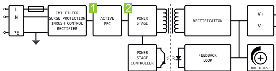
Fig. 23: Block diagram of E models
