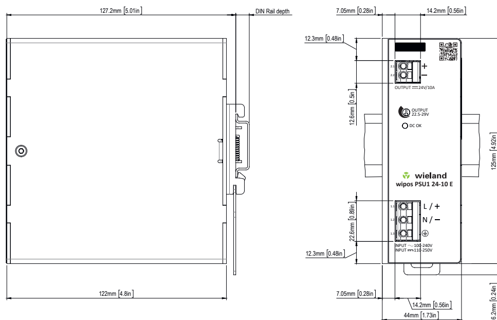
Fig. 16: Dimension drawing of wipos PSU1 24-10 E
